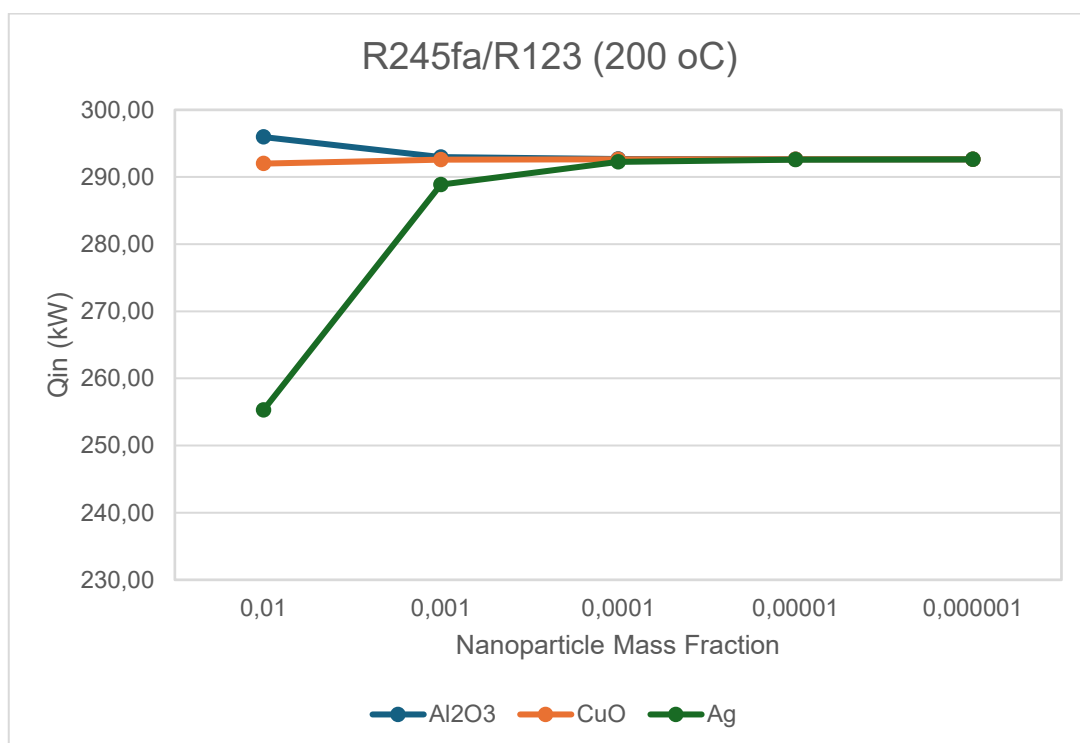
Figure 4.20: Heat Absorbed vs. Nanoparticle Mass Fraction for R245fa/R1233zd
