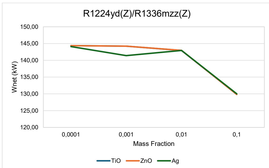
Figure 4.25: Net Power Output Variation with Nanoparticle Mass Fraction for R1224yd(Z)/R1336mzz(Z)
